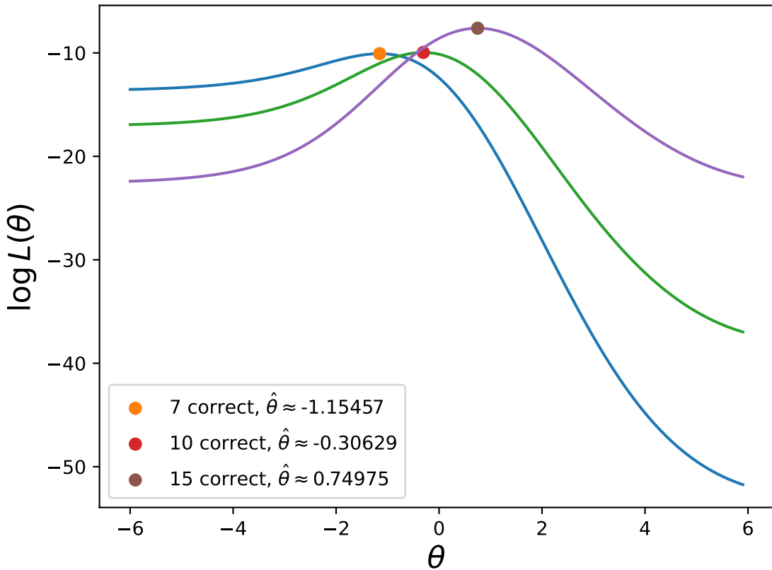
brent (4 avg. evals)
